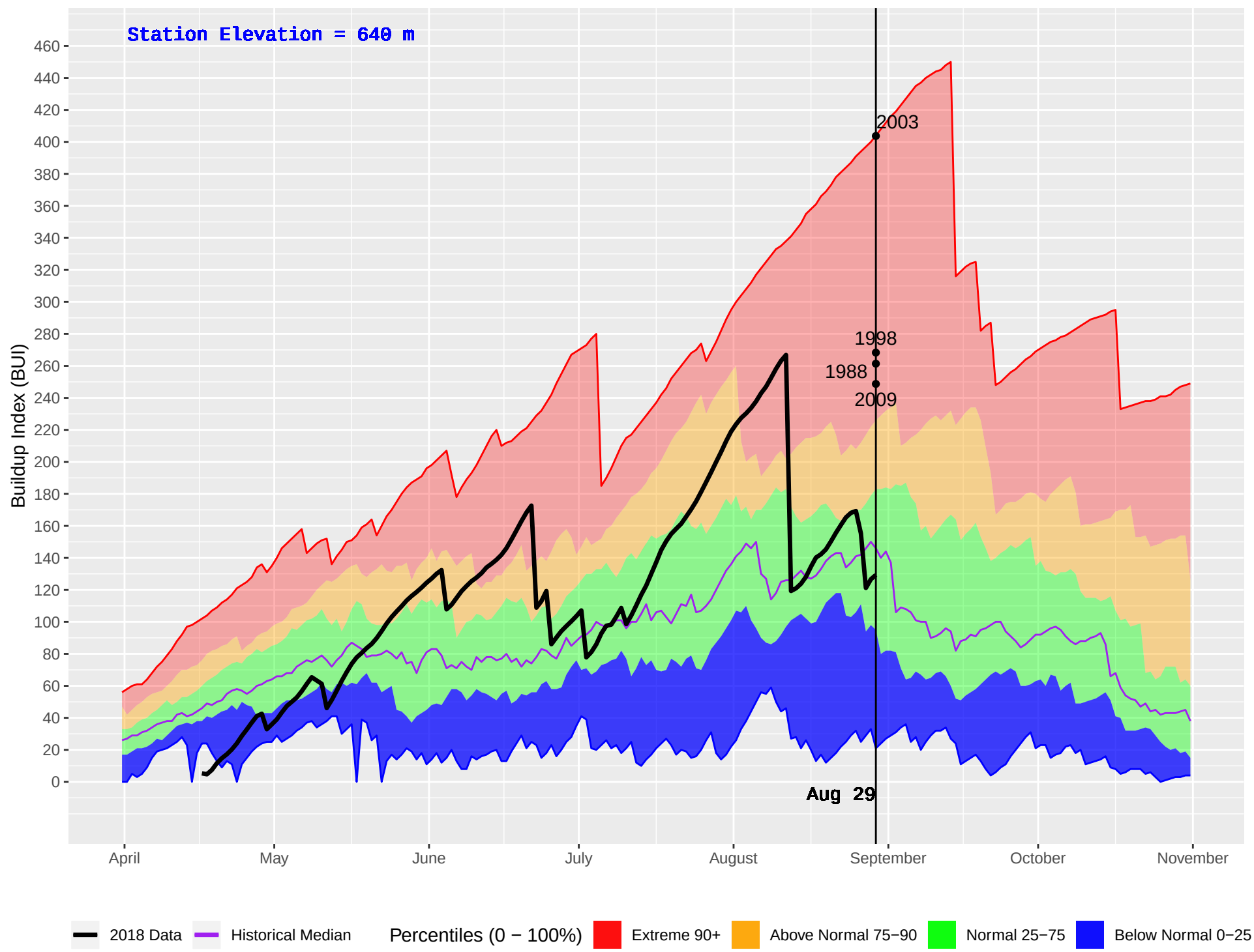
MERRITT HUB (294) : Historical (1978–2016) and Current (2018) Daily Buildup Index (BUI)
