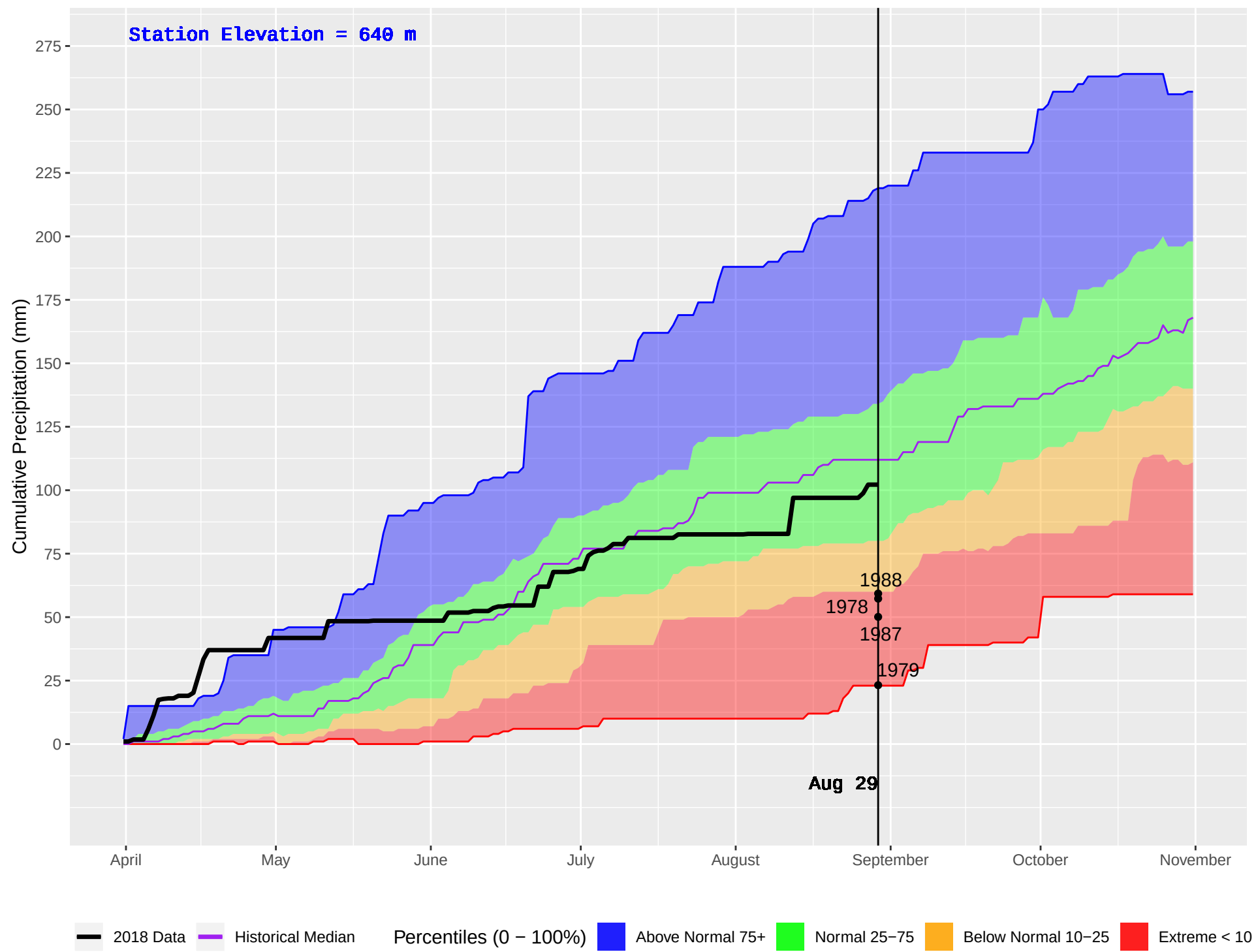
MERRITT HUB (294) : Historical (1978–2016) and Current (2018) Daily Cumulative Precipitation
