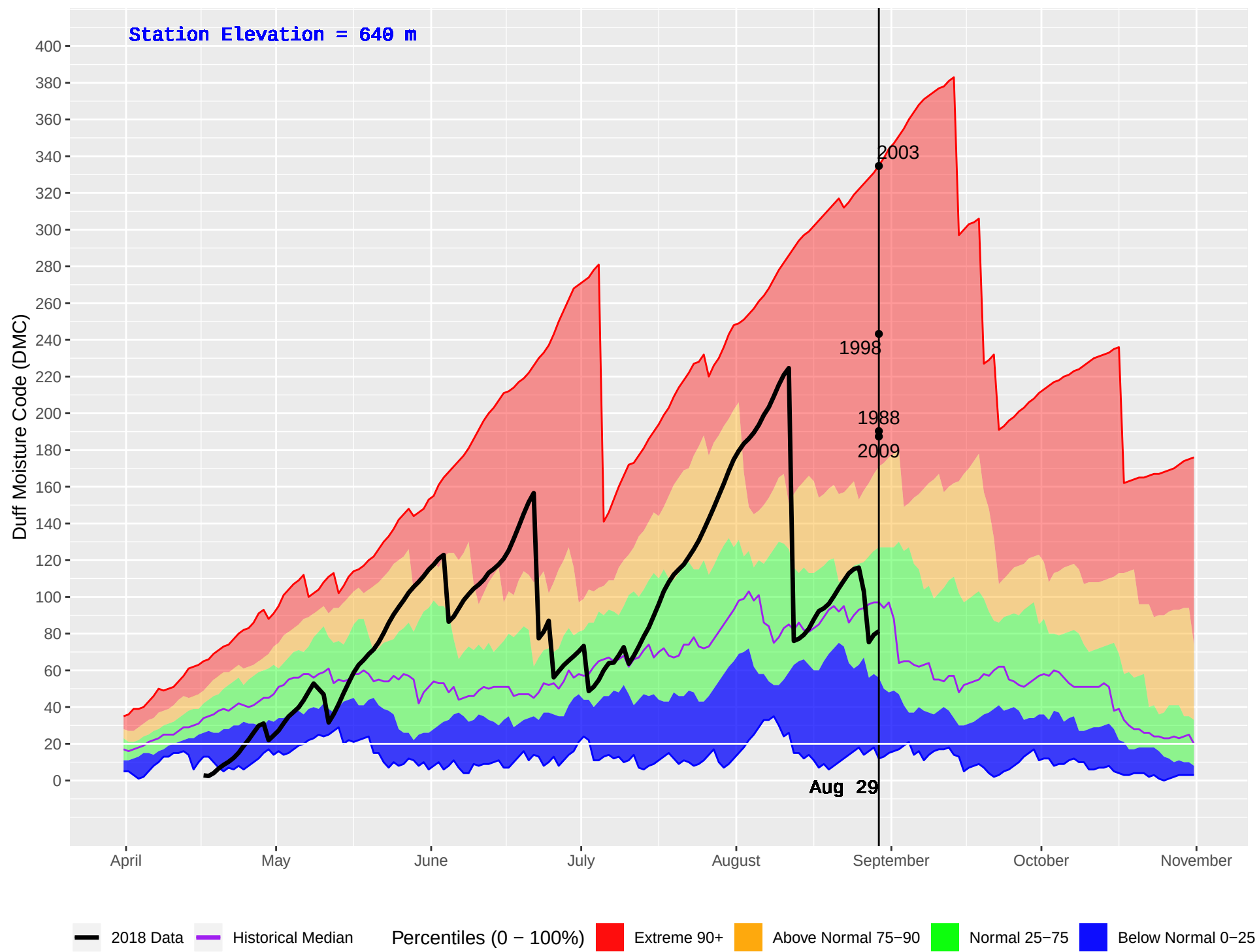
MERRITT HUB (294) : Historical (1978–2016) and Current (2018) Daily Duff Moisture Code (DMC)
