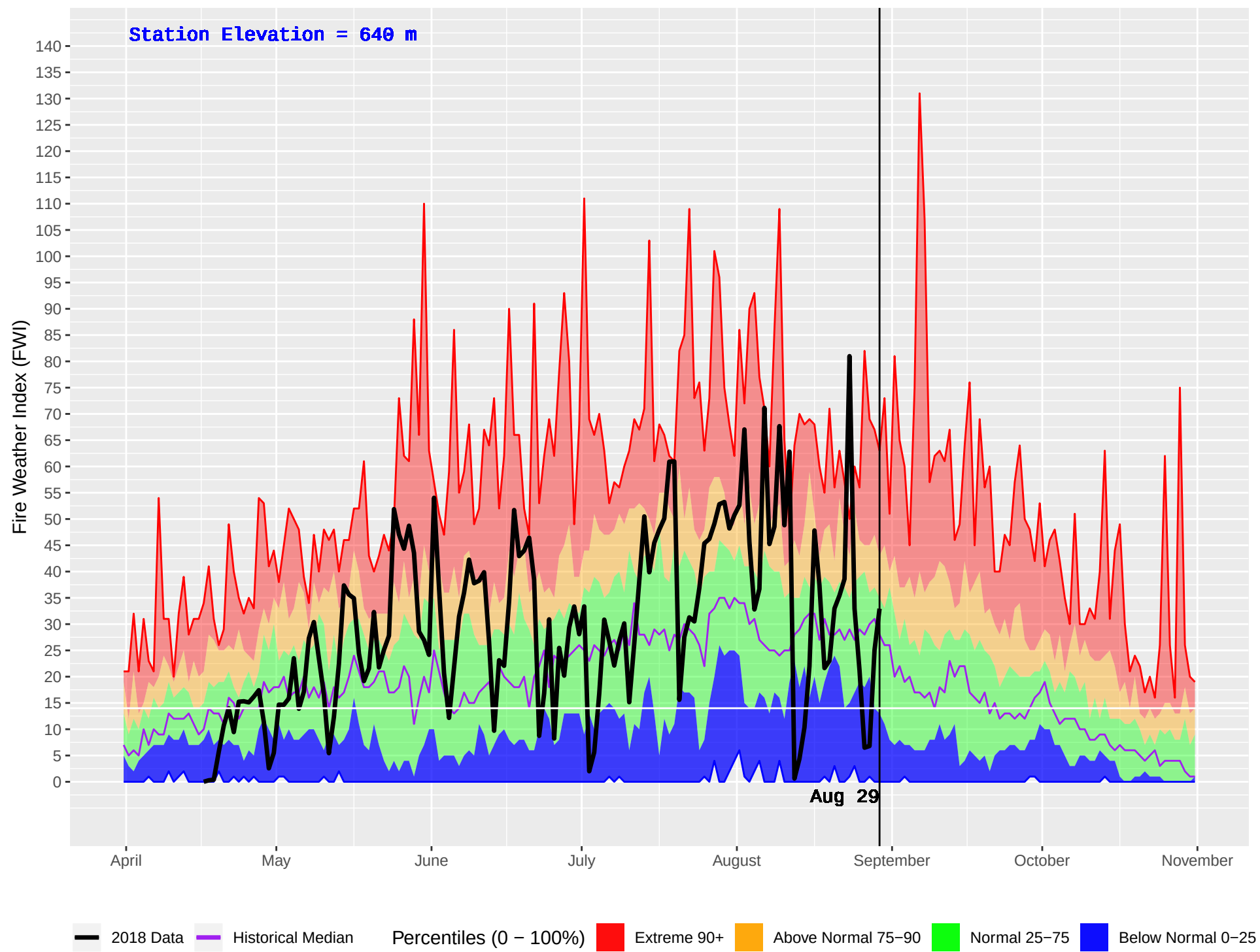
MERRITT HUB (294) : Historical (1978–2016) and Current (2018) Daily Fire Weather Index (FWI)
