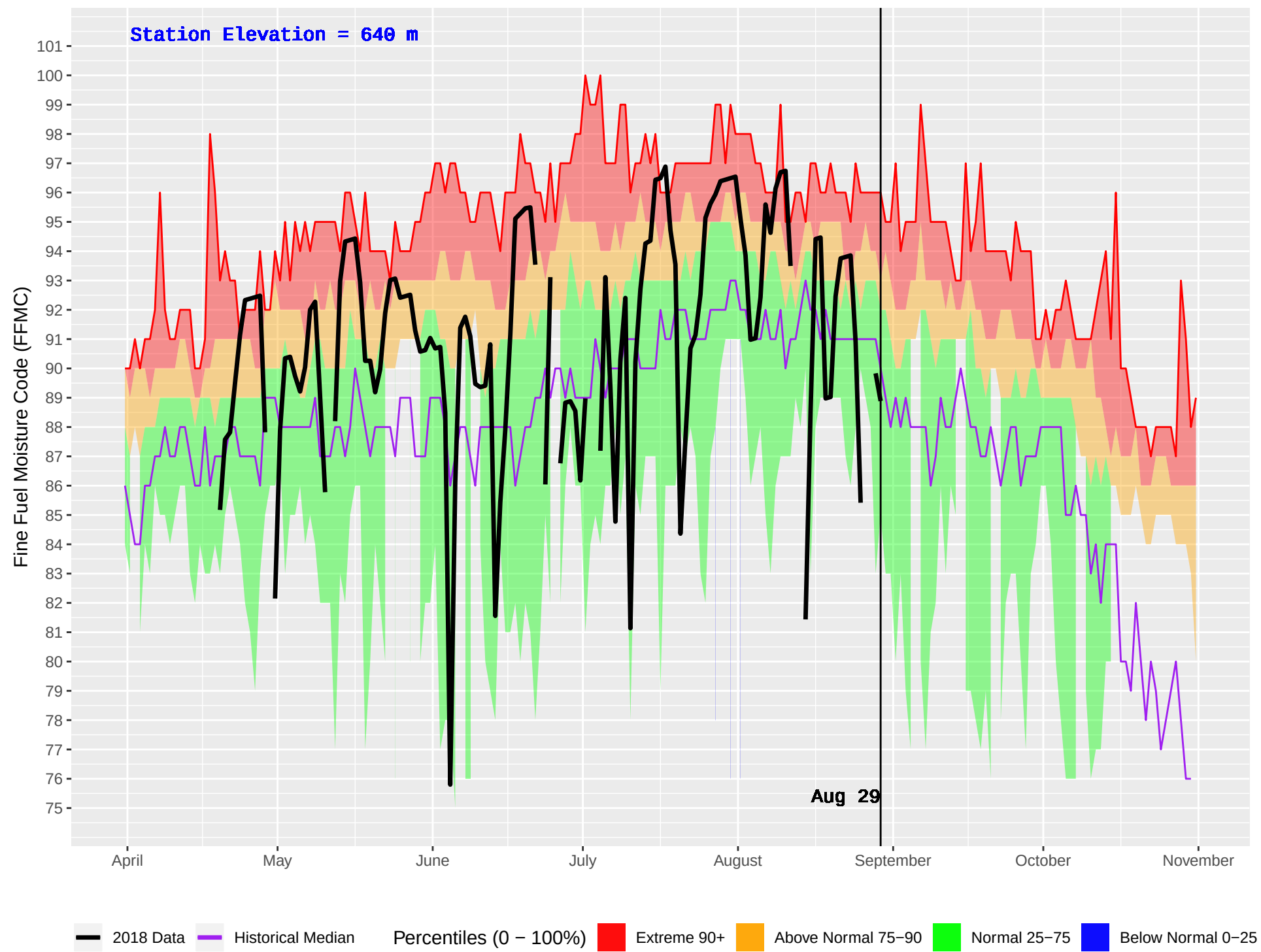
MERRITT HUB (294) : Historical (1978–2016) and Current (2018) Daily Fine Fuel Moisture Code (FFMC)
